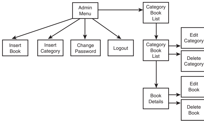
Figure 28.2 The administrator view of the Book-O-Rama system allows insertion, editing, and deletion of books and categories.
