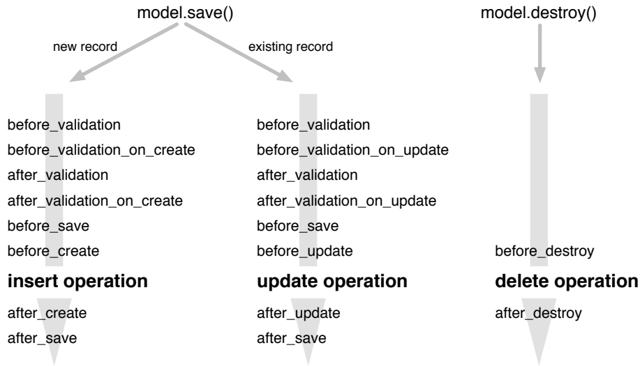
Figure 19.2: Sequence of Active Record callbacks
