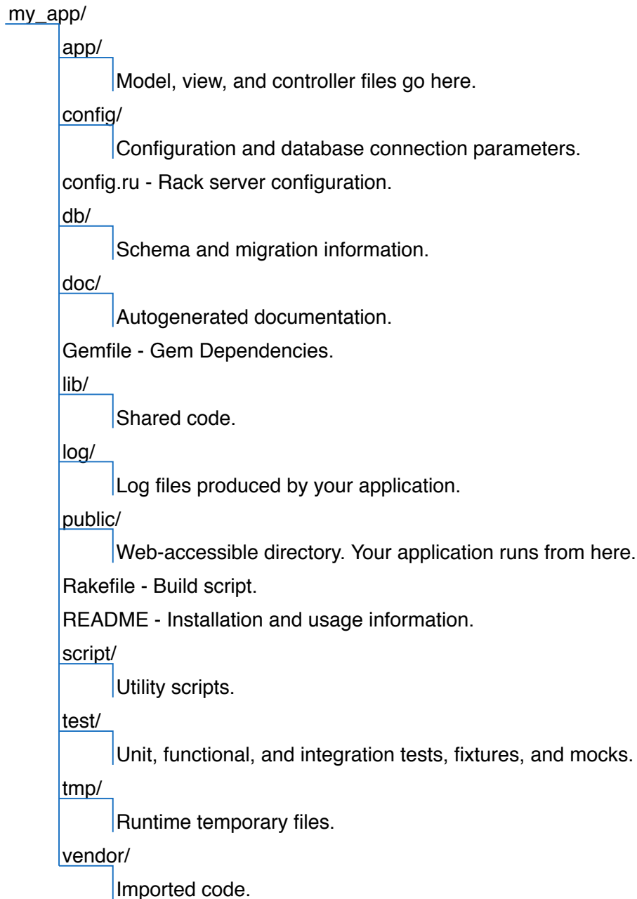
Figure 18.1: All Rails applications have this top-level directory structure.
