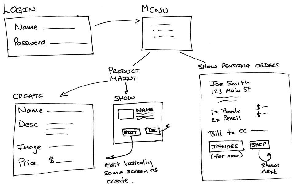
Figure 5.2: Flow of seller pages
