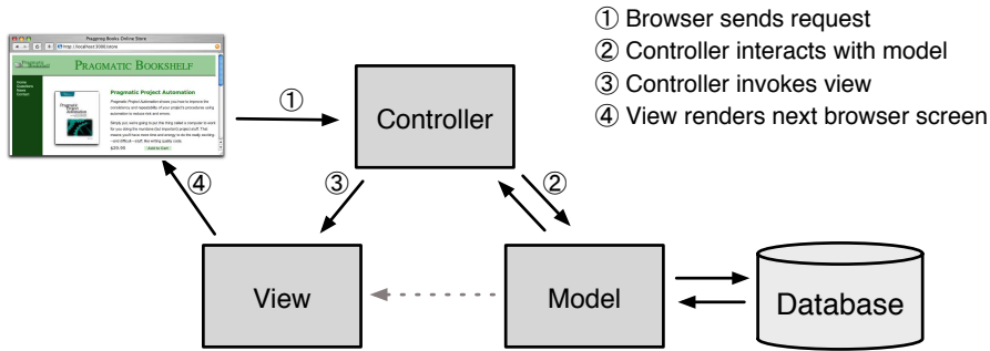
Figure 3.1: The Model-View-Controller architecture
