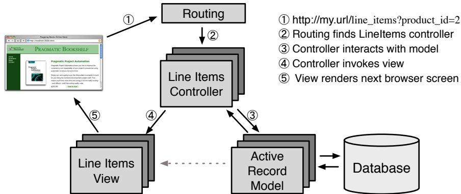
Figure 3.2: Rails and MVC
