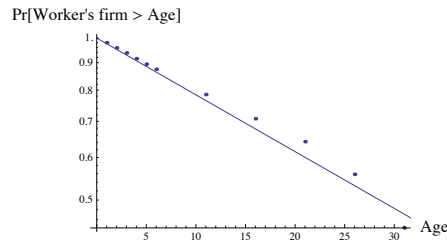
Figure 25: Counter cumulative distribution of employment by firm age in years in the U.S. (line) and in the model (dots); source: BLS (BDM), available online
