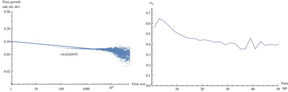
Figure 21: Dependence of the standard deviation of g on (a) firm size and (b) firm age
