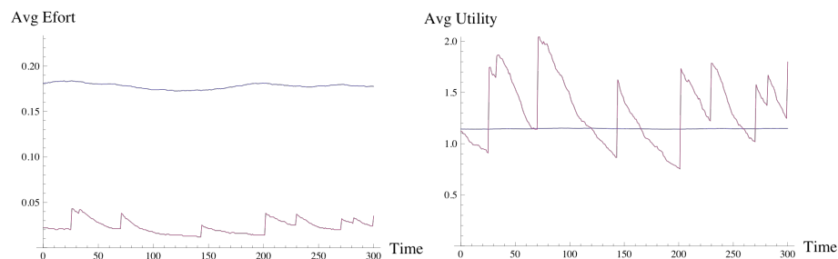
Figure 8: Typical time series for (a) average effort level in the population (blue) and in the largest firm (magenta), (b) average utility (blue) and in the largest firm (magenta)
