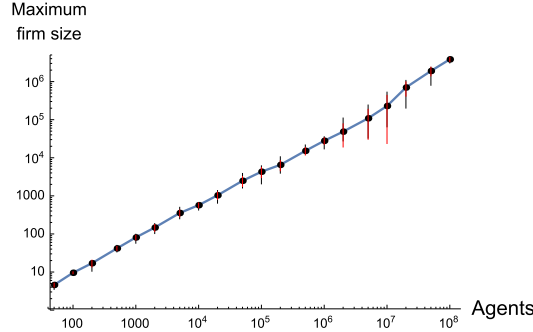
Figure 28: Largest firm size realized as a function of the number of agents
