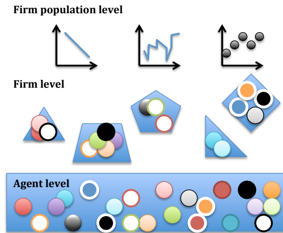
Figure 29: Multi-level schematic of firm formation from agents
