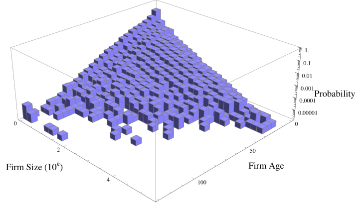
Figure 16: Histogram of the steady-state distribution of firms by \log(S) and age in the model. Note that log probabilities decline approximately linearly as a function of age and \log(S) . Many of the largest firms in the model are relatively young ones that grow rapidly, much like in the U.S. economy (e.g., Luttmer 2011, figure 1).
