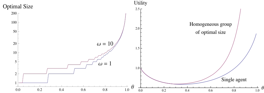
Figure 3: Optimal size (a) and utility (b) in homogeneous teams versus \theta ; a = b = 1 ; \omega = 1, 10
